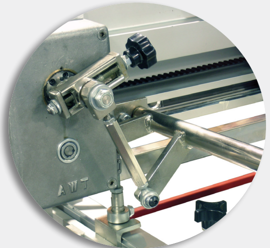
Exclusive upfront peel system gives operator quick and convenient control of peel rate setting.
