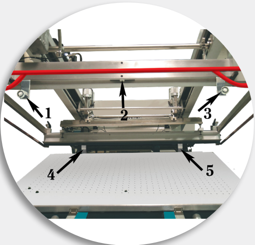
Five-point masterframe lock-in: Ensures critical registration for multicolor printing. Wraparound safety bar (red) protects press operator.
