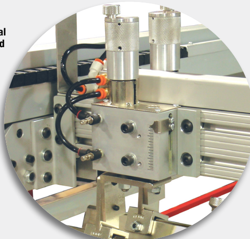
Squeegeelizer - Pneumatic chopper assembly equalizes squeegee and floodbar pressure across entire print area.
